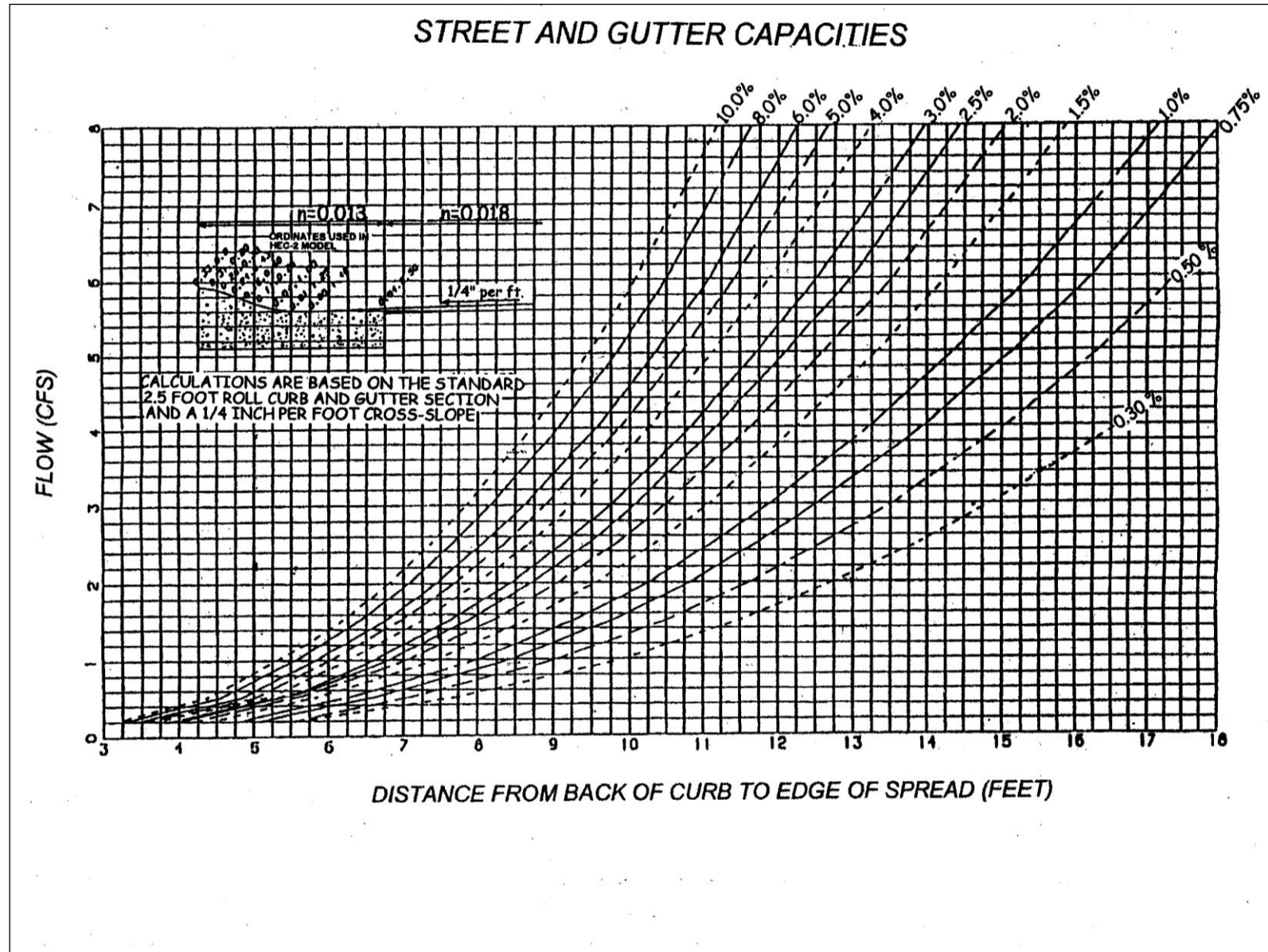
FIGURE 4-1: Street and Gutter Capacities (continuous grade)
