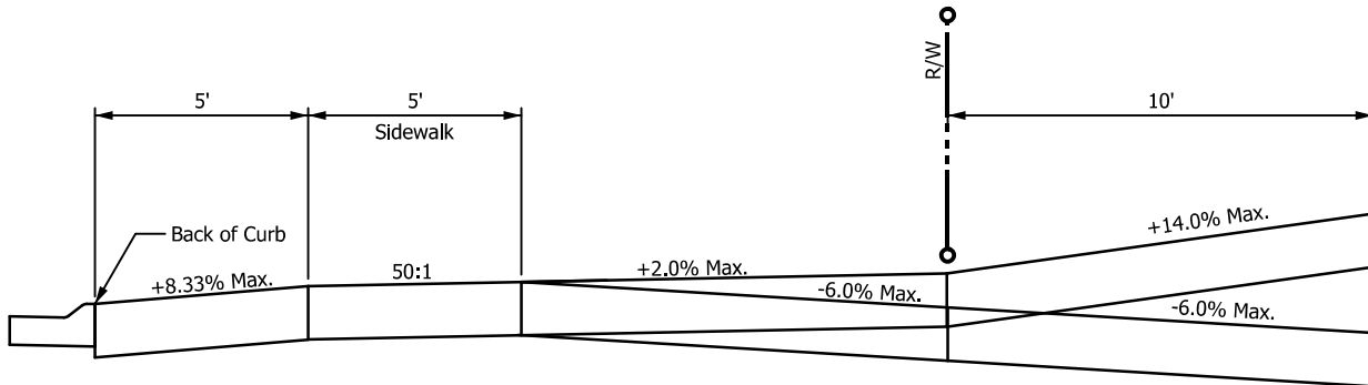
CURB AND GUTTER WITH SIDEWALK
